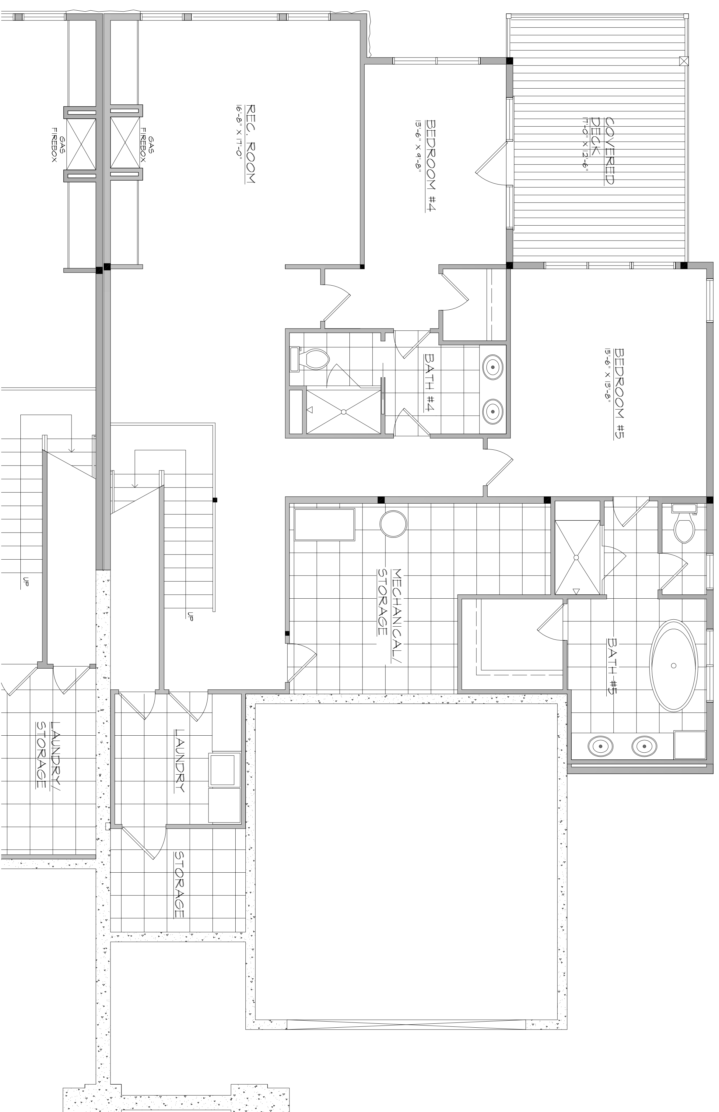
NORTH RESIDENCE LOWER LEVEL FLOOR PLAN 1797 FINISHED SQUARE FEET
